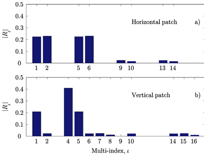
Fig. 2. Spherical vector wave expansion coefficients of (a) horizontal patch antenna and (b) the vertical patch antenna.
