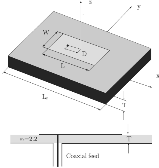
Fig. 1. The horizontal patch antenna. The vertical patch is obtained by a rotation around the y-axis towards the x-axis.
