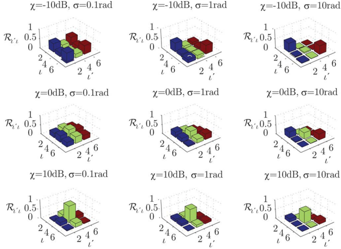
Fig. 6. Elements of the covariance matrix R_{\iota'\iota} , where \iota = \{\tau ml\} is the multipole multi-index where 2 = \{2, -1, 1\} , 4 = \{2, 0, 1\} and 6 = \{2, 1, 1\} .
