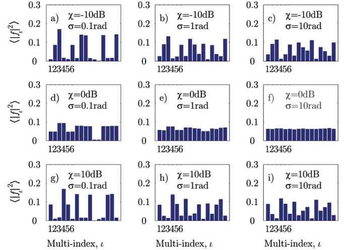
Fig. 3. Average mode power versus mode index for the random field simulated according to (41).
