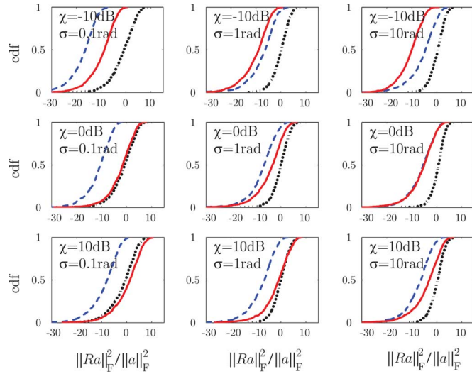
Fig. 4. Cumulative distribution functions (cdf) of the normalized instantaneous gain of the horizontal patch (---), the vertical patch (—) and the conjugate matched antennas, (···). Results are shown for different values of the channel cross-polarization ratio, \chi and the \sigma -parameter of the Laplace distribution of the AoA.
