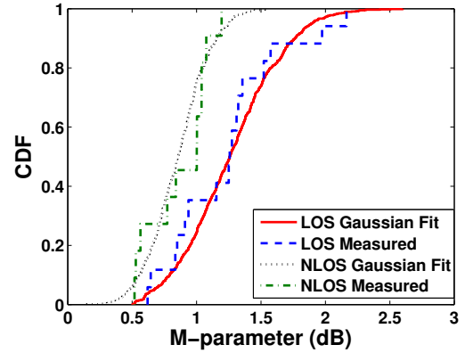
Fig. 14: CDF of m - parameter (dB) at mm-wave band.
